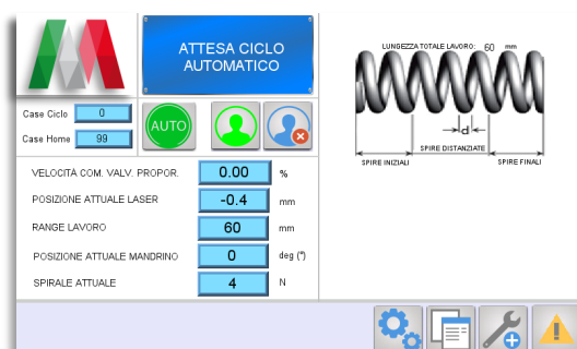
CNC Coiling Program Touch Screen
